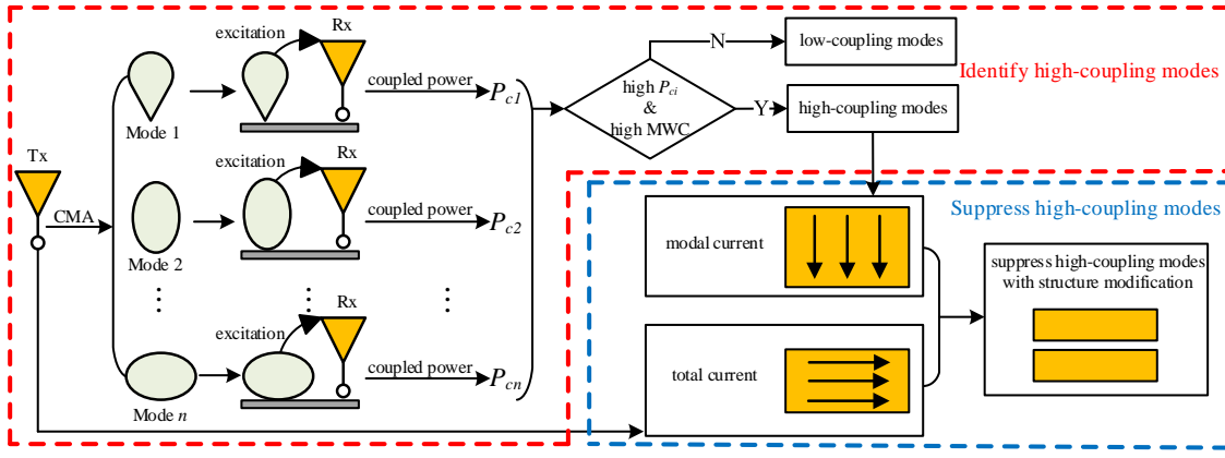
Fig. 1. The flowchart of the proposed self-decoupling method. Two main steps include the high-coupling modes identification and the high-coupling modes suppression.
