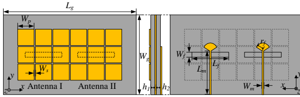
Fig. 2. Configurations of the MTS antenna array. ( L_g = 92.6 , L_f = 25 , L_m = 28.9 , W_g = 56.3 , W_f = 1.5 , W_m = 1.1 , W_p = 11.3 , W_s = 0.8 , h_1 = 3 , h_2 = 0.5 , g = 0.5 , r_f = 5.4 . Unit: mm.)
