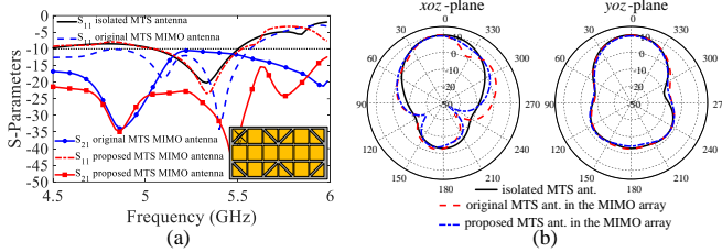
Fig. 3. (a) S-Parameters of the isolated MTS antenna and the MTS antenna in the MIMO array; (b) Far-field patterns at 5.3 GHz for the isolated MTS antenna, the original MTS antenna in the MIMO array and the proposed MTS antenna in the MIMO array.
