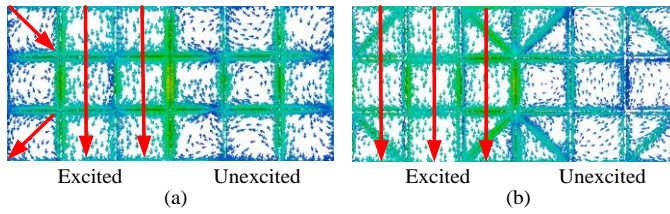
Fig. 5. Current distributions of the MTS antennas at 5.3 GHz (a) initial antennas; (b) self-decoupled antennas.
