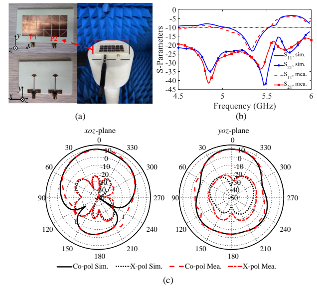
Fig. 6. (a) Photographs of the fabricated prototype and the measurement setup; (b) Simulated and measured S-parameters of the self-decoupled MTS antenna array; (c) Simulated and measured radiation patterns at 5.3 GHz.
