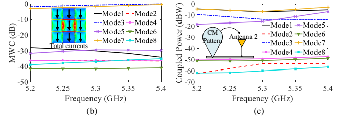
Fig. 4. (a) Modal currents and modal fields of the MTS antenna; (b) MWCs of the first eight modes of the MTS antenna; (c) Coupled power of each mode to the Rx MTS antenna.
