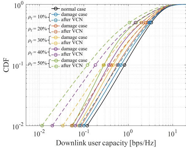
Fig. 4: CDF of downlink user capacity as a function of \rho_f .
