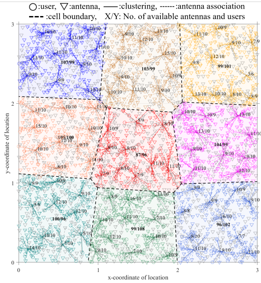
Fig. 1: An example of multi-cell DAS after antenna failure.
