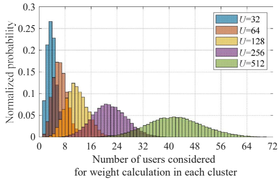
(a) User-centric
