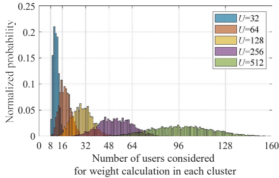
(b) Cluster-centric
